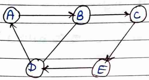
Fig: Directed Graph
