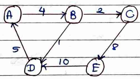
Fig: weighted directed graph
