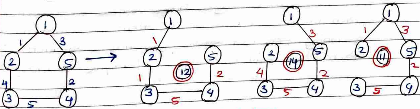
Spanning tree
