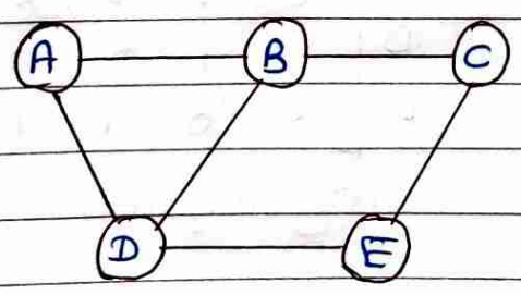
Fig: undirected graph
